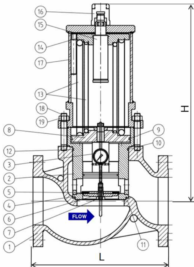
EXTERNAL DIMENSIONS
